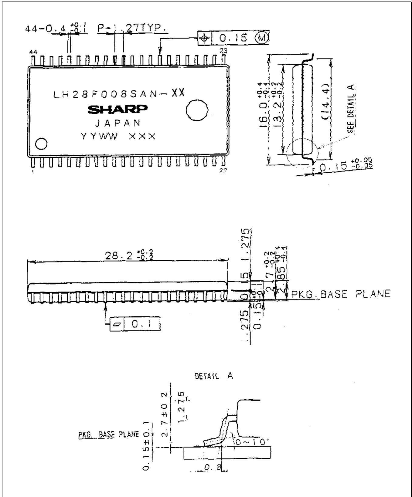
44-Lead SOP
